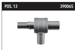
KBZ 500 Dust extraction rotor for dry drilling
