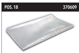
Replacement pouch set f. cyclone filter LxW: 600x300 mm, 150µ; PU 25 St.
