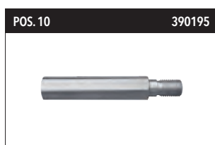
KBZ 770 core bit extension
